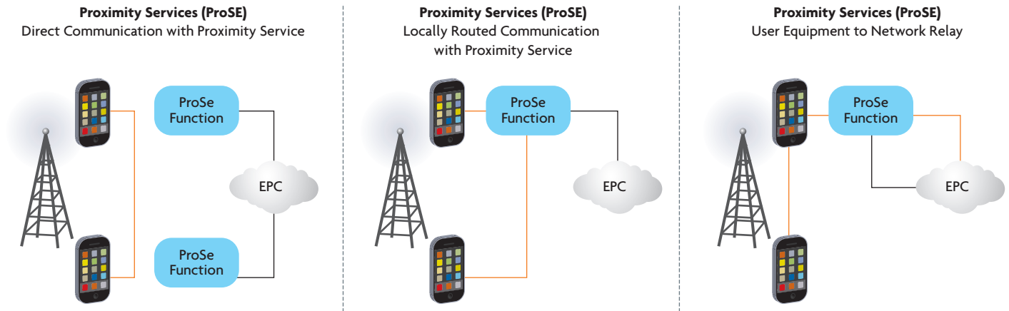
Figure 6. R13 LTE-D Enhancements
