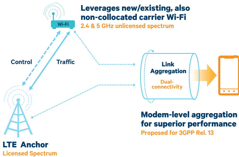
Fig. 4: LTE – Wi-Fi link aggregation for carrier Wi-Fi networks
