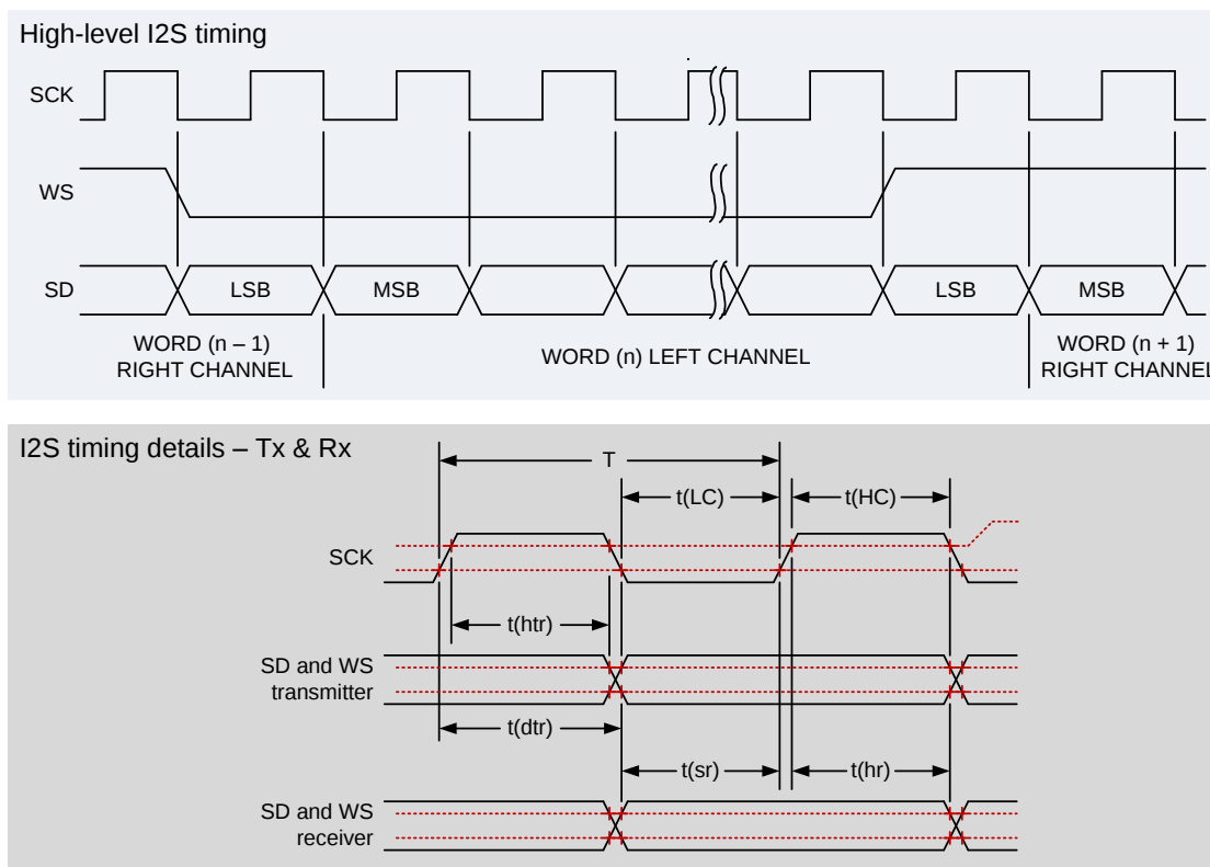
Figure 3-13 I 2 S timing diagram
