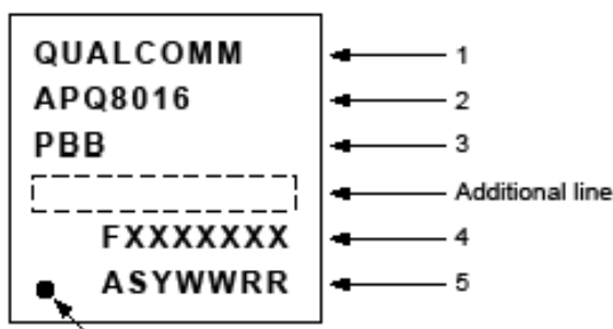
Figure 4-2 APQ8016E device marking (top view, not to scale)
