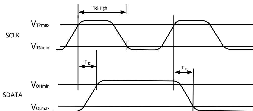
Figure 3-18 Waveform
