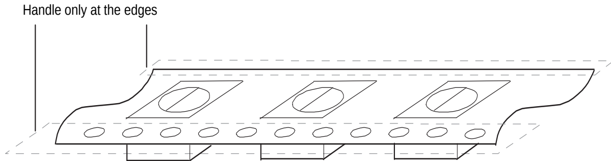
Figure 5-2 Tape handling
