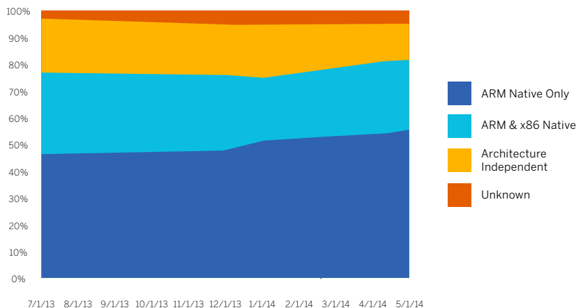
FIGURE 5: CODE FORMAT OVER TIME FOR TOP 100 APPS US GOOGLE PLAY STORE
