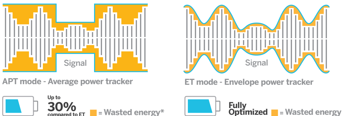
FIGURE 9: ENVELOPE TRACKING BENEFITS
