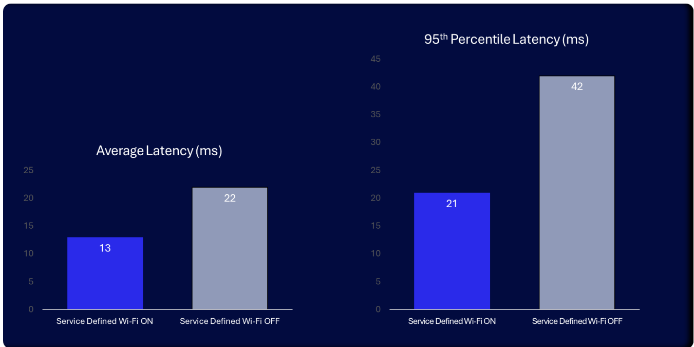
Figure 12 Latency (Average and 95 th Percentile) Classroom Use Case
