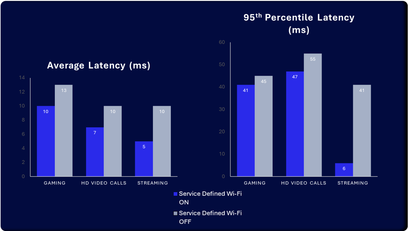
Figure 9 Latency (Average and 95 th Percentile) Multi-client Multi-application Use Case
